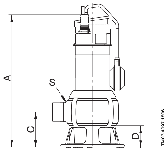
Fig. 36 Pump dimensions
