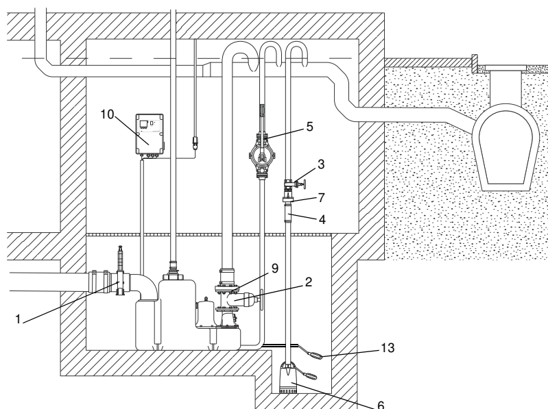
Fig. 25 Accessories for Multilift MLD
