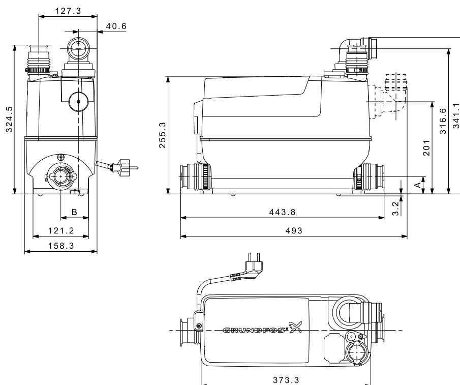
Fig. 37 Dimensional drawings, Sololift2 C-3
