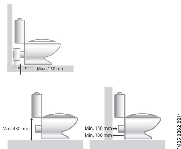
Fig. 7 Measurements to be observed
