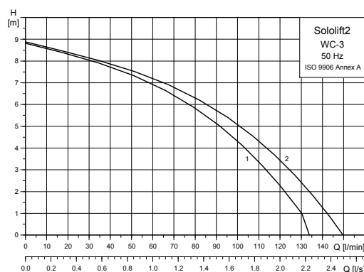
Fig. 18 Performance curves, Sololift2 WC-3
