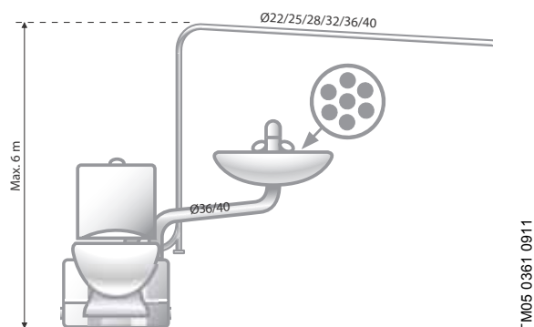
Fig. 6 Example of installation
