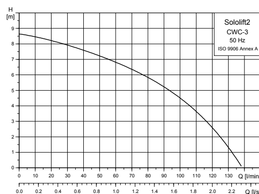
Fig. 26 Performance curves, Sololift2 CWC-3
