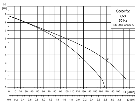
Fig. 36 Performance curves, Sololift2 C-3
