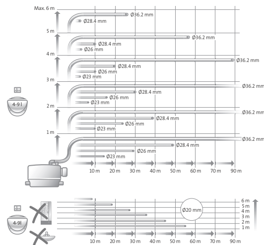
Fig. 22 Maximum lengths of vertical and horizontal discharge pipes
