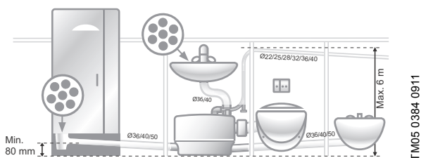
Fig. 23 Example of installation
