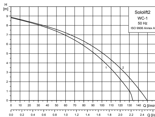
Fig. 9 Performance curves, Sololift2 WC-1
