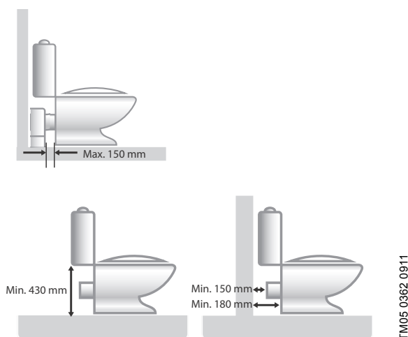
Fig. 15 Measurements to be observed
