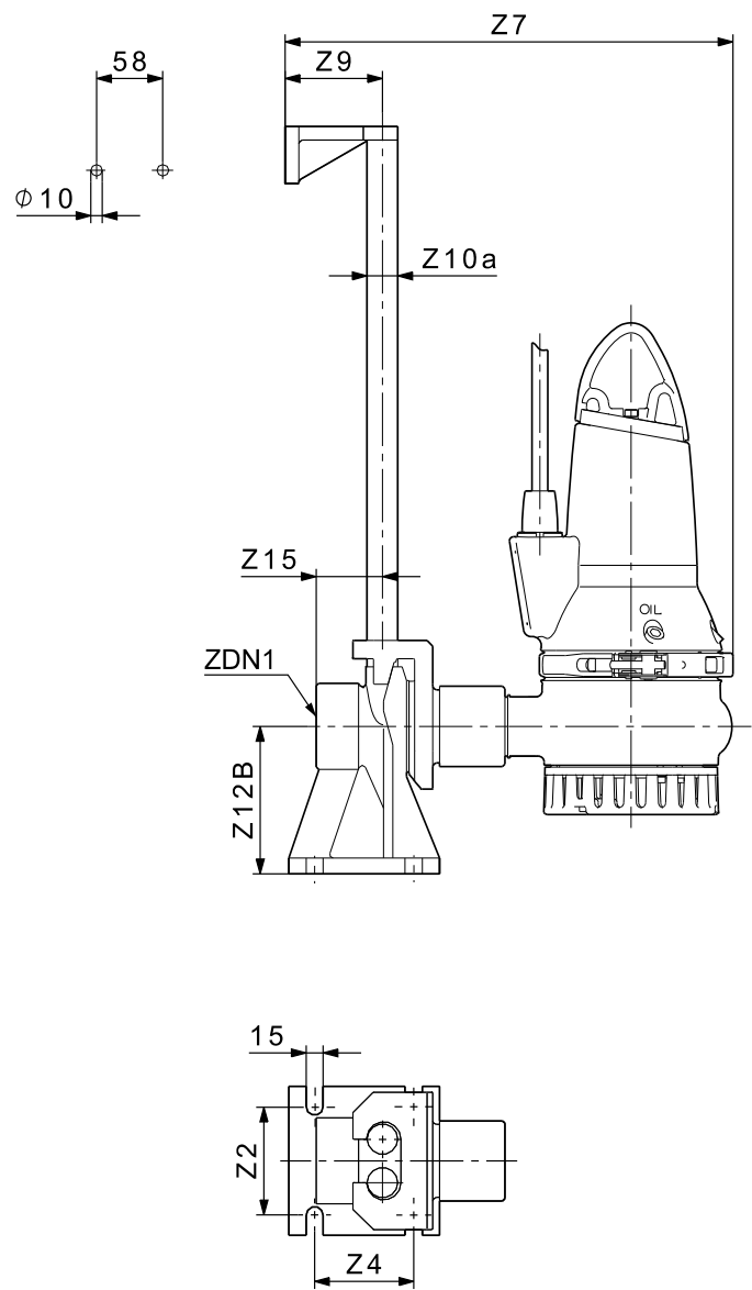
Fig. 32 One-pump installation on auto-coupling
