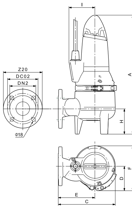
Fig. 48 Free-standing installation
