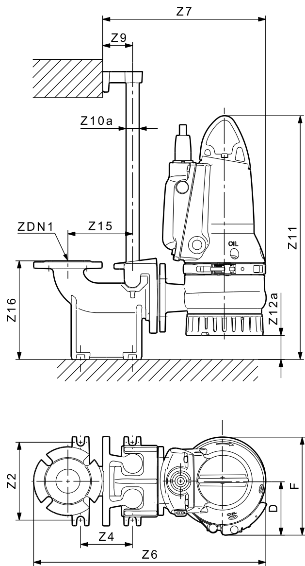
Fig. 35 One-pump installation on auto-coupling
