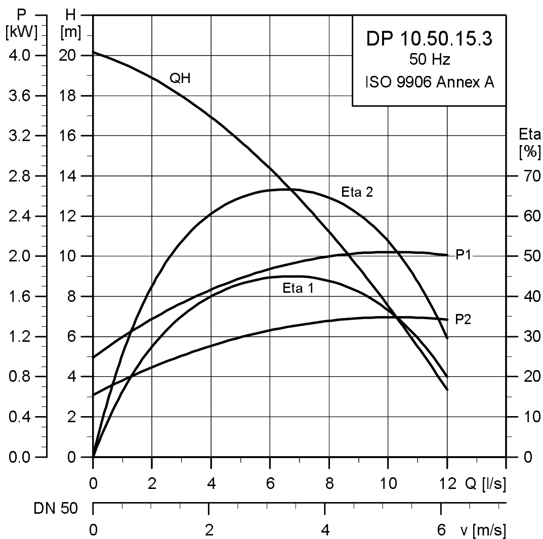
Performance curves, DP10.50.15.(E).(Ex).3
