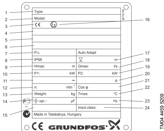
Fig. 3 DP, EF, SL1 and SLV AUTO ADAPT pumps
