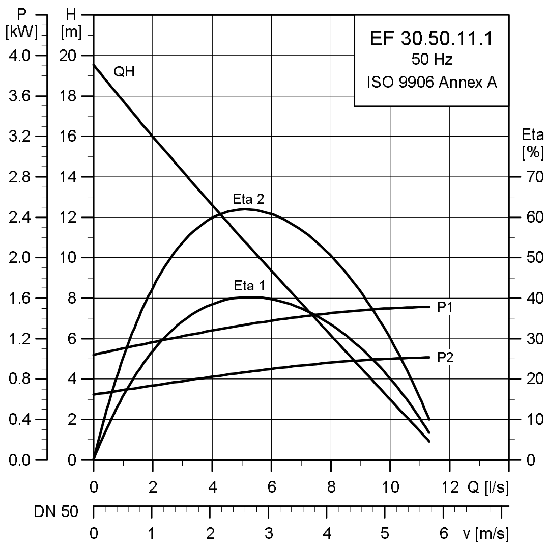
Performance curves, EF30.50.11.(E).(Ex).1
