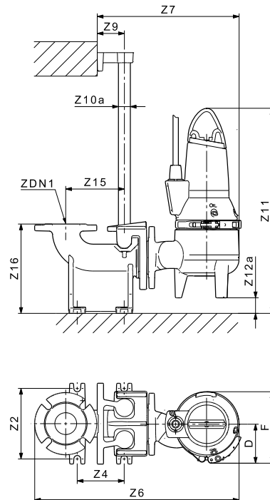
Fig. 45 One-pump installation on auto-coupling
