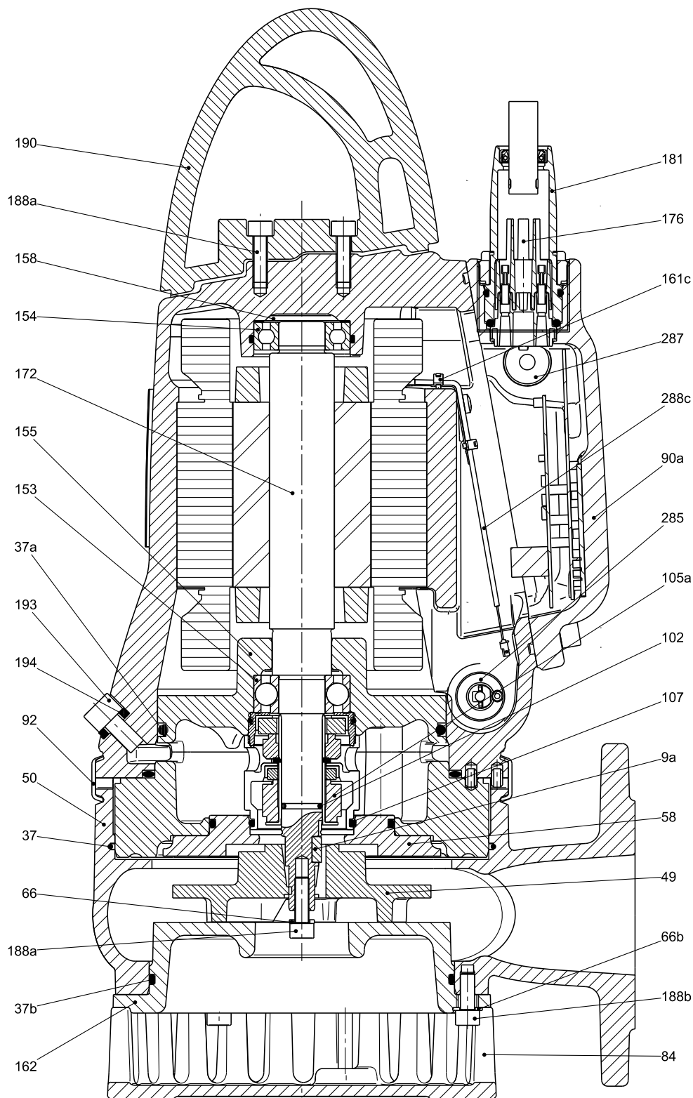
Fig. 13 Sectional drawing, DP10.65.26 AUTO ADAPT
