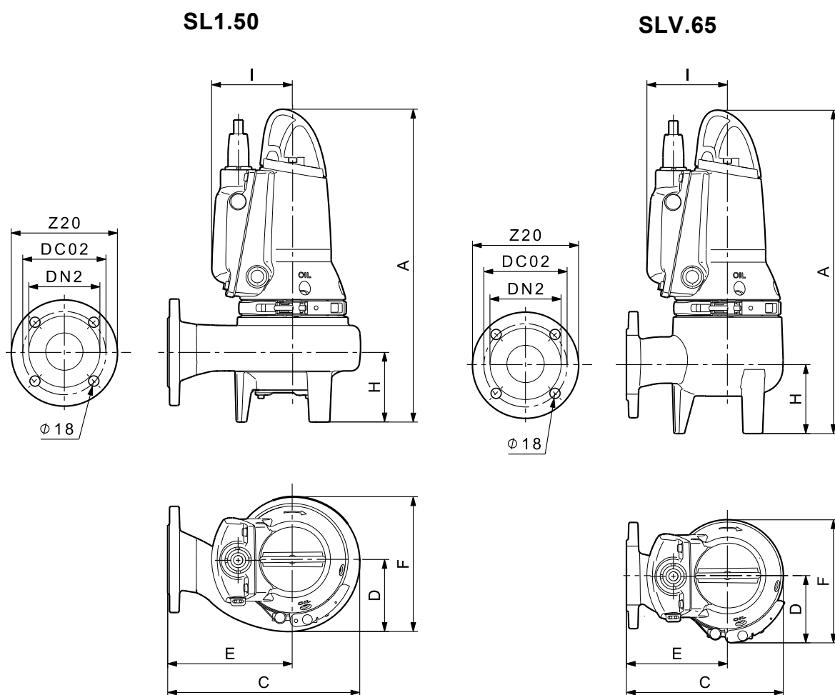
Fig. 49 Free-standing installation
