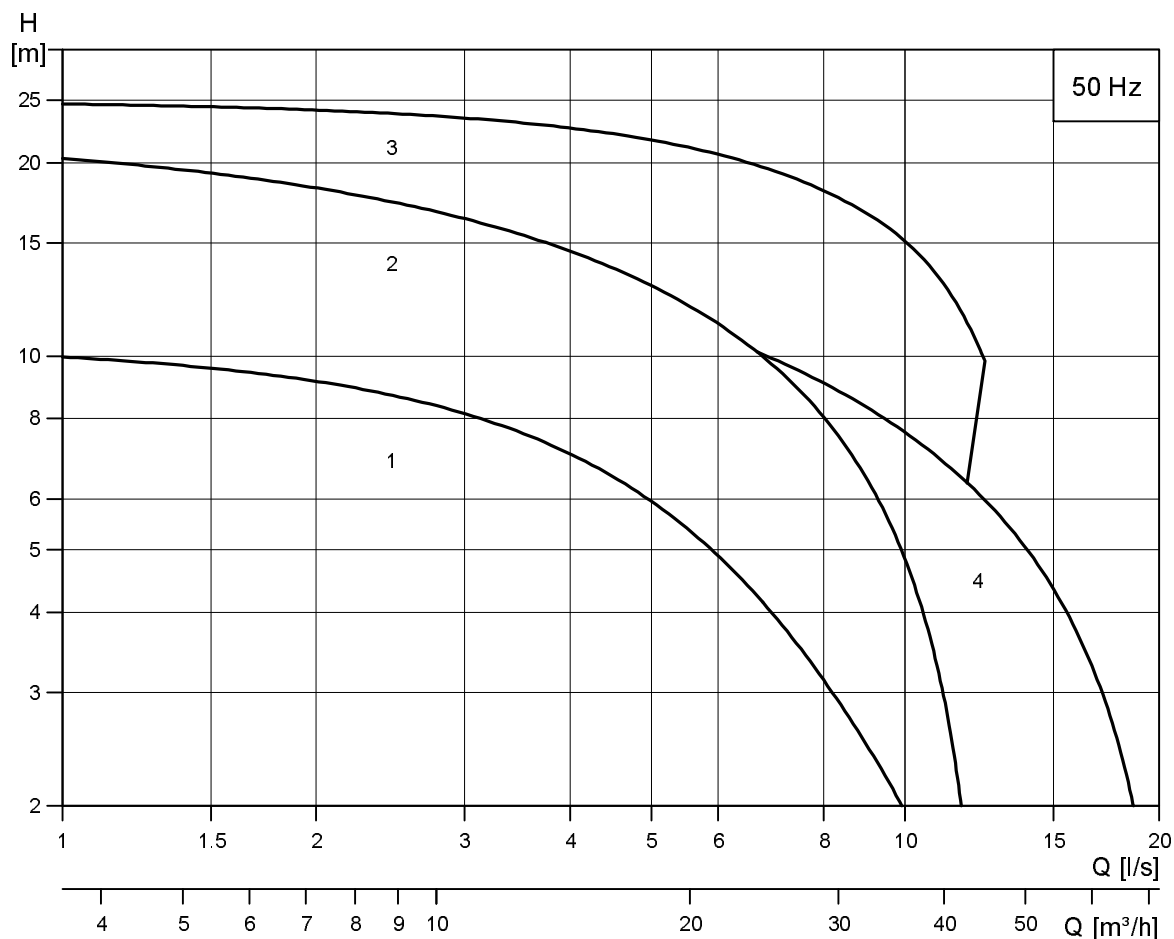
Fig. 4 Performance range
