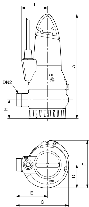
Fig. 39 Free-standing installation
