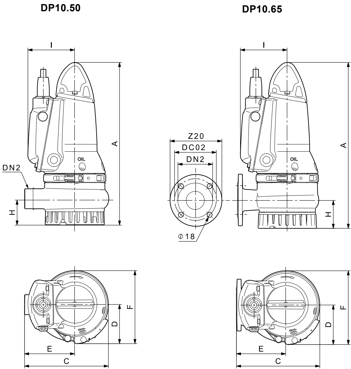
Fig. 41 Free-standing installation
