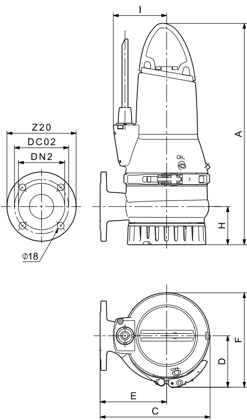
Fig. 40 Free-standing installation
