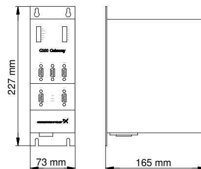
Fig. 24 Dimensional sketch
