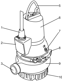
Fig. 1 Pump DP 10.50
