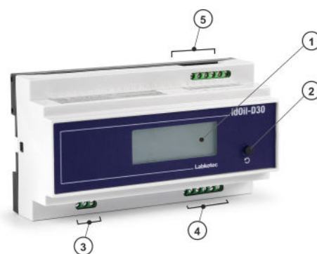
Figure 27. Features of the idOil control unit
