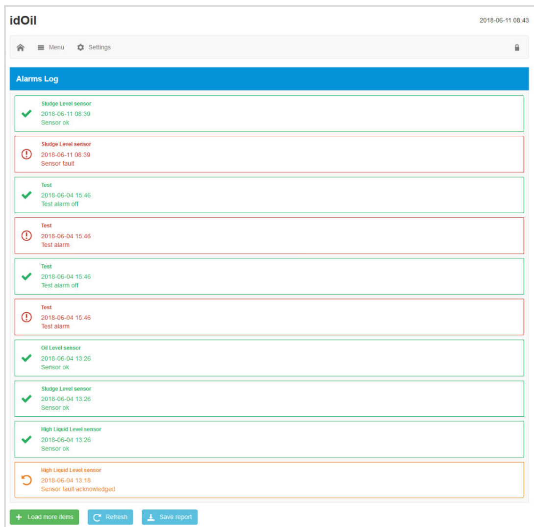
Figure 30. Alarm log
