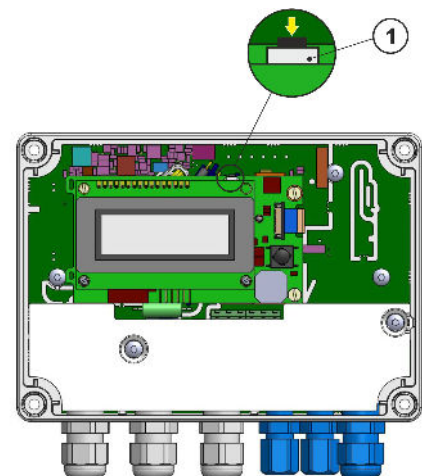
Figure 17. Sensor identification button.
